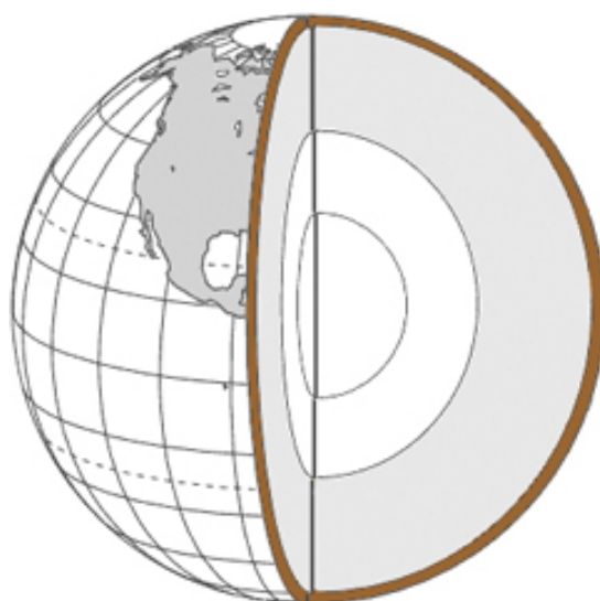
Crust
