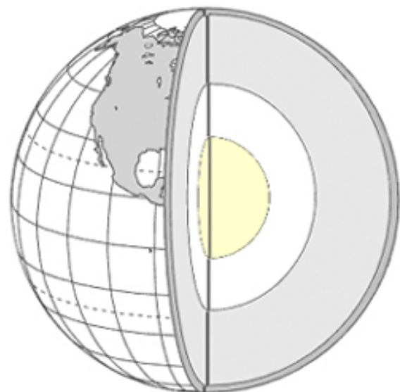
Inner Core
