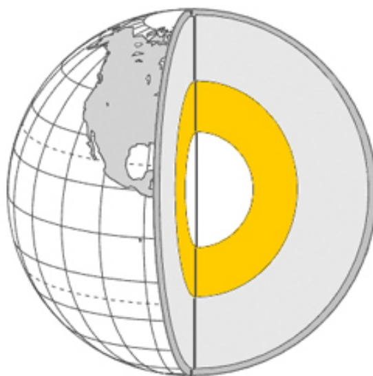
Outer Core
